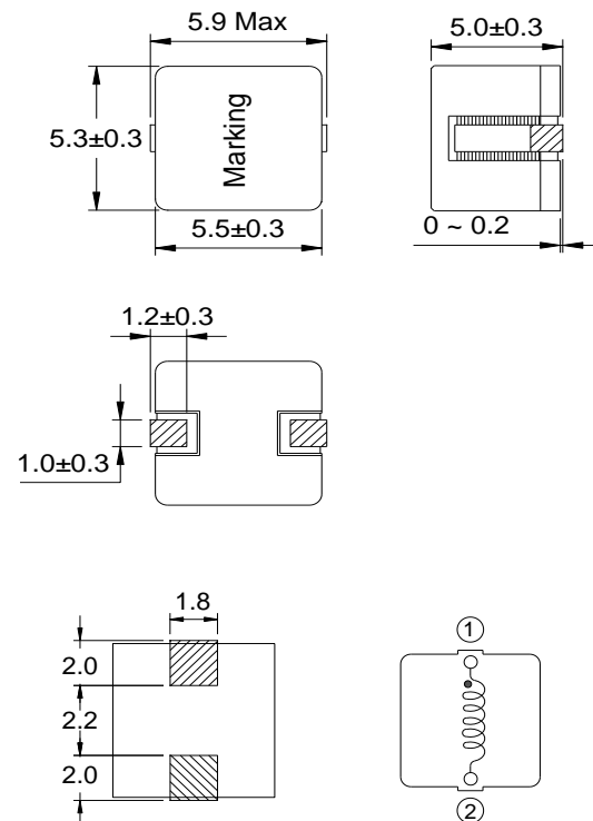
Typical Land Pattern
